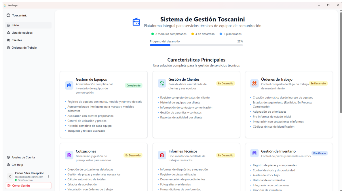
Figura 3.56 Dashboard Recepción
